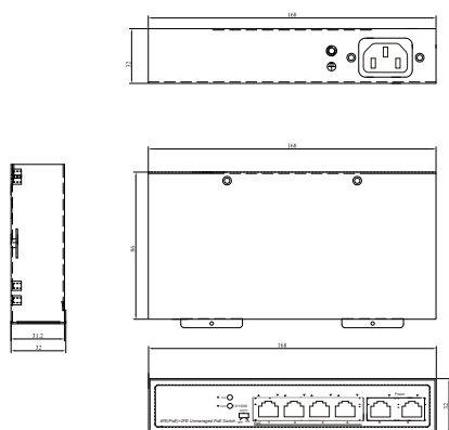
NSW2010-6T-POE-IN
