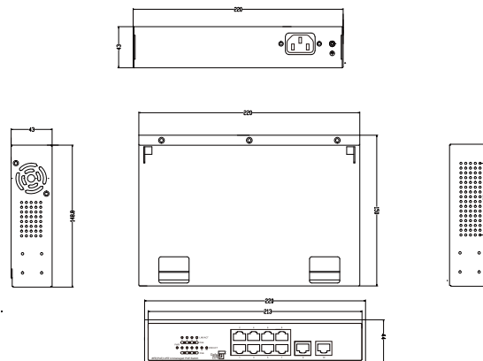
NSW2010-10T-POE-IN
